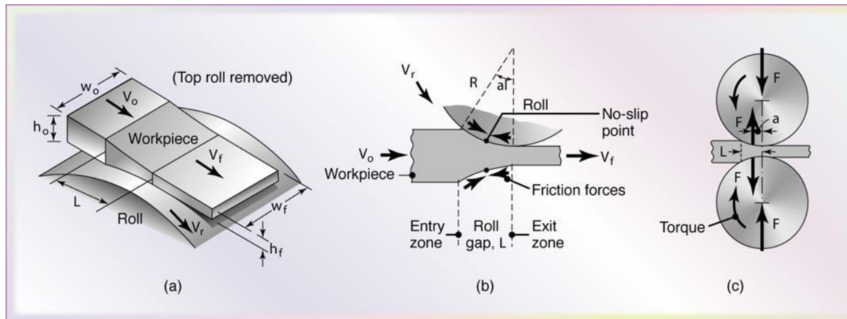
Figure 13.2 (a) Schematic illustration of the flat-rolling process. (b) Friction forces acting on strip surfaces. (c) Roll force, F , and the torque, T , acting on the rolls. The width of the strip, w , usually increases during rolling, as shown later in Fig. 13.5.
